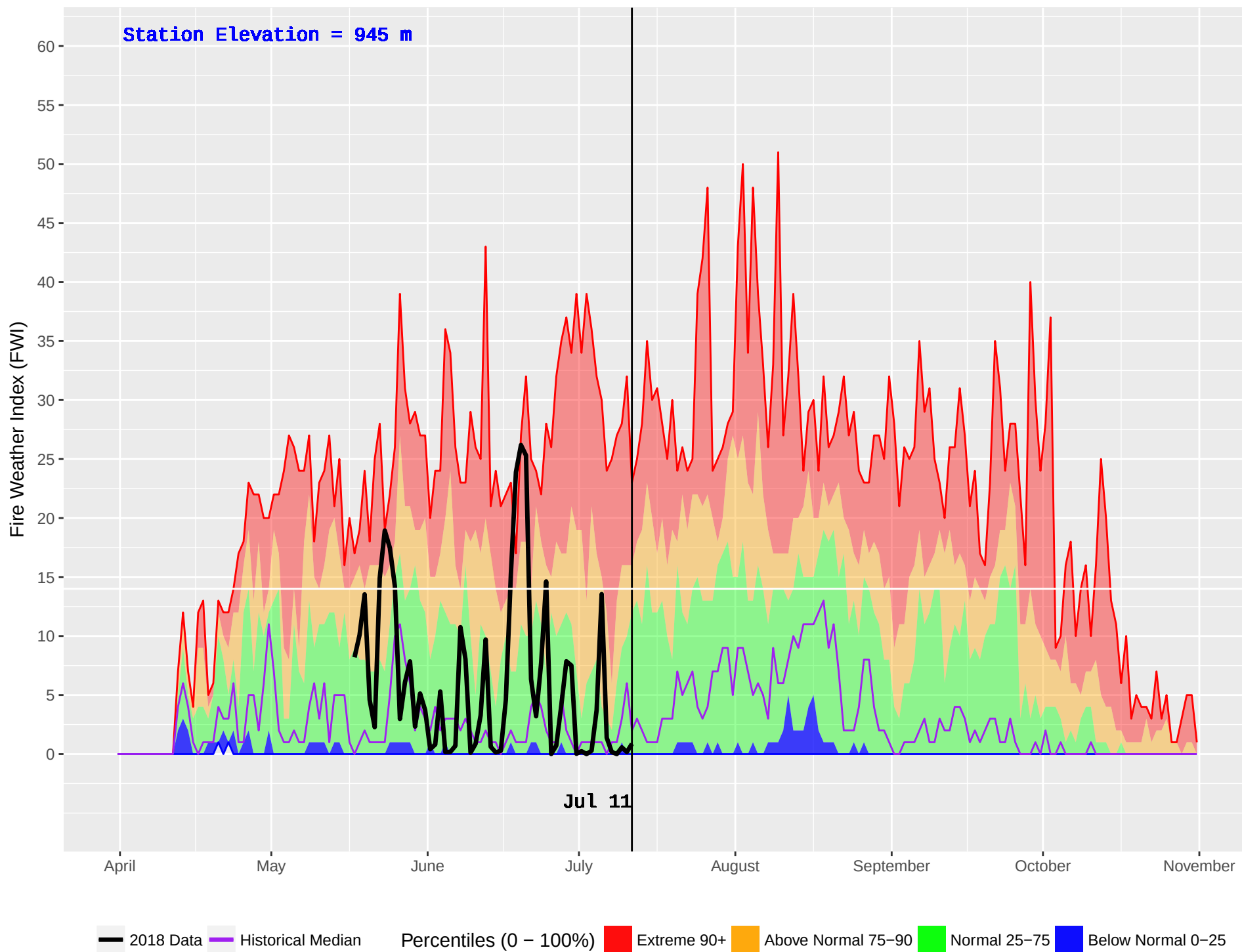
BOWRON HAGGEN (193) : Historical (1986–2016) and Current (2018) Noon Fire Weather Index (FWI)
