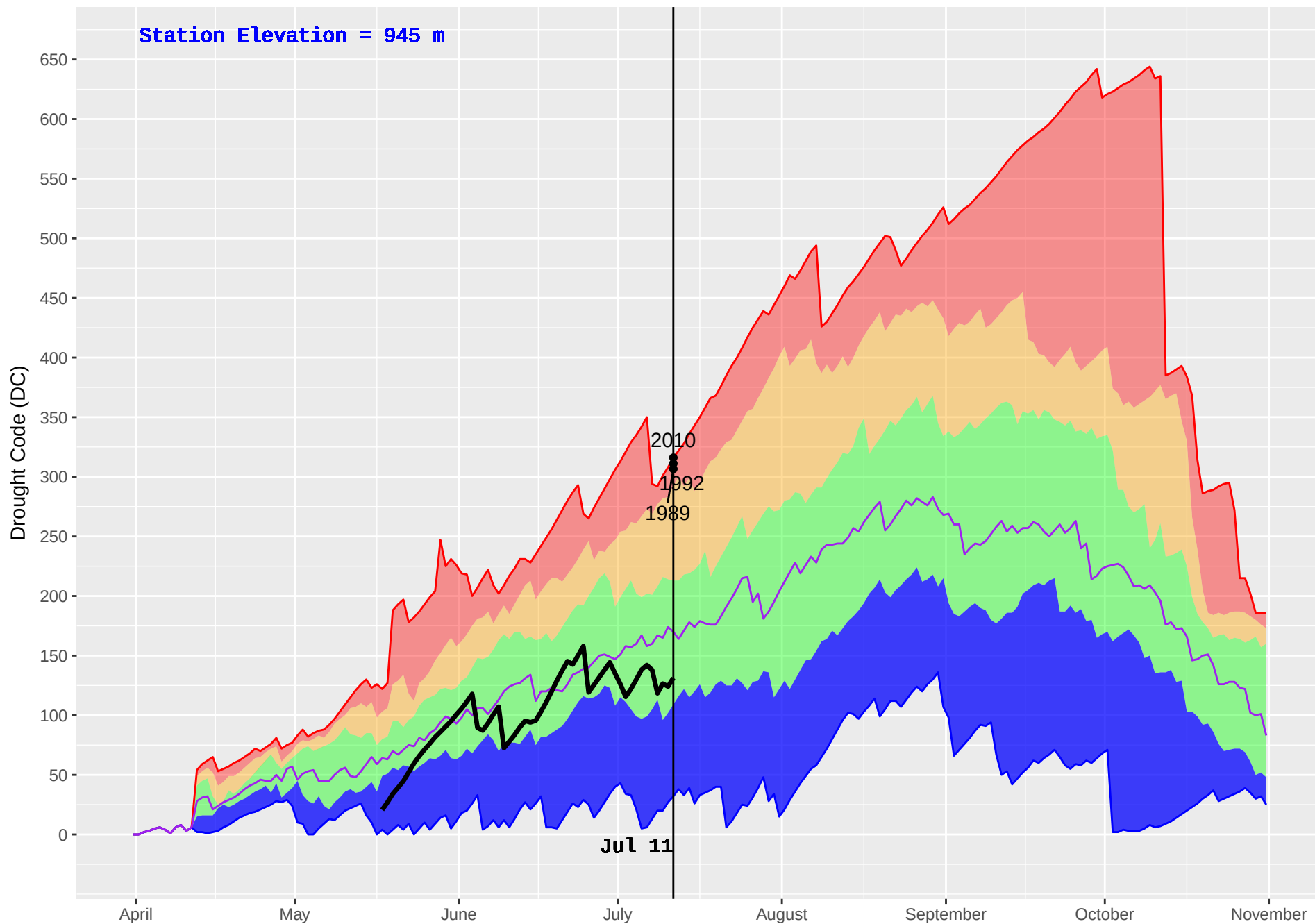
BOWRON HAGGEN (193) : Historical (1986–2016) and Current (2018) Noon Drought Code (DC)
