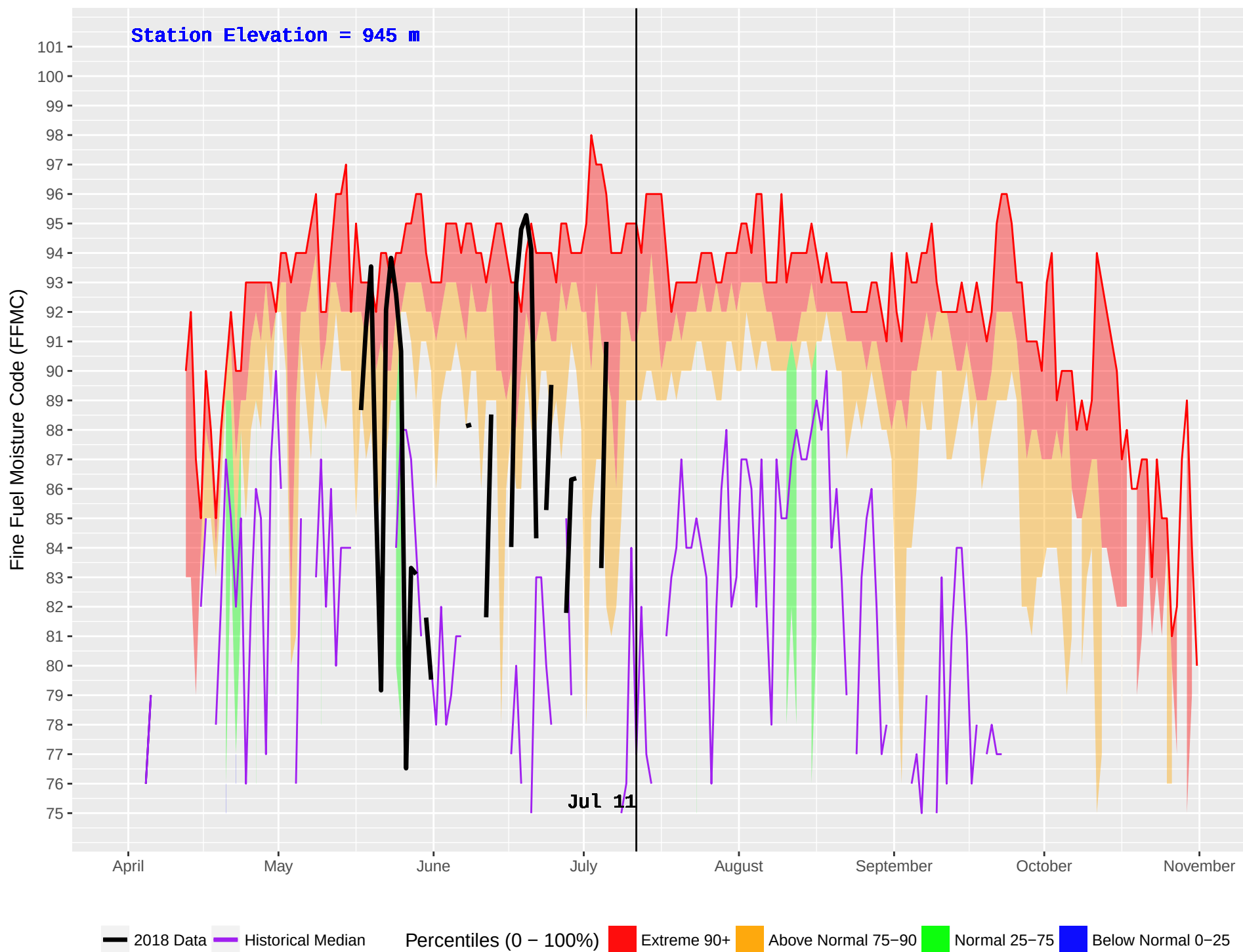
BOWRON HAGGEN (193) : Historical (1986–2016) and Current (2018) Noon Fine Fuel Moisture Code (FFMC)
